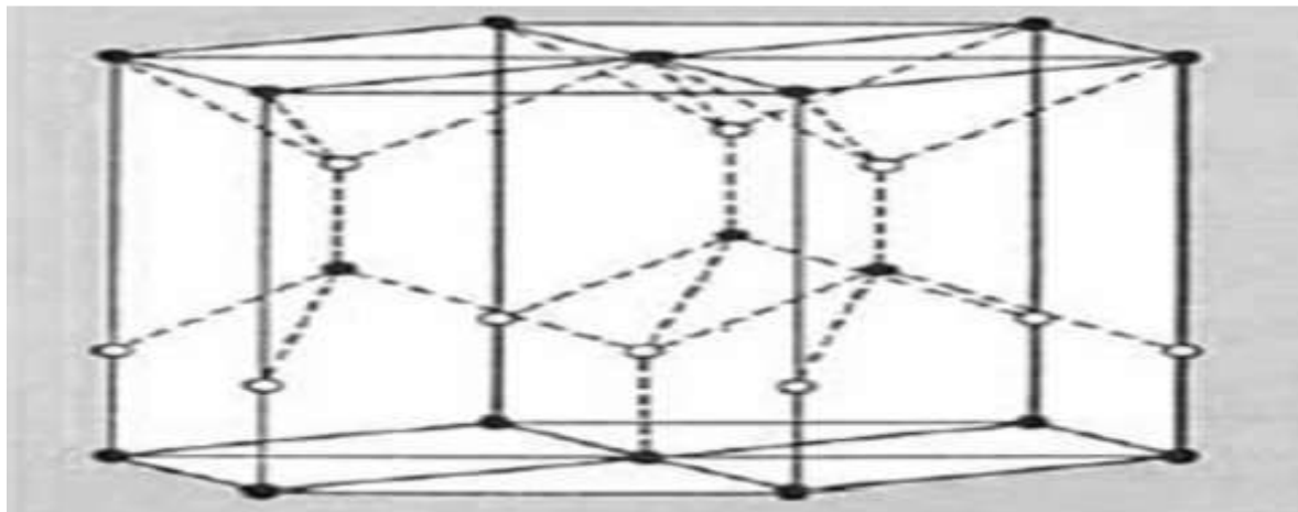
Figure 1.1 The crystal structure of ZnO (shaded circles indicate the positions of oxygen atoms while the open circles indicate the positions of the zinc atoms) Source: Gazene 2006
