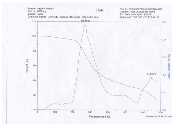
Fig (5): The TG / DTG thermograms of (R-COOHMP-Co) complex
