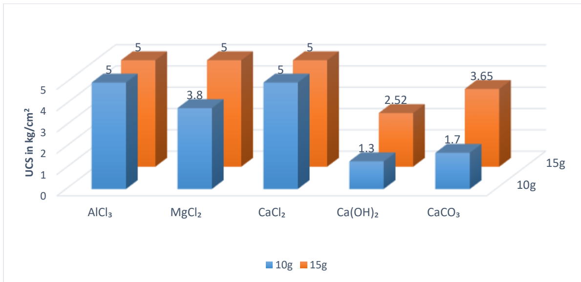
Figure 4: Penetrometer confirmation (in kg/cm 2 ) of the stabilization of 10g and 15g each of the erosive soil using the chemicals
