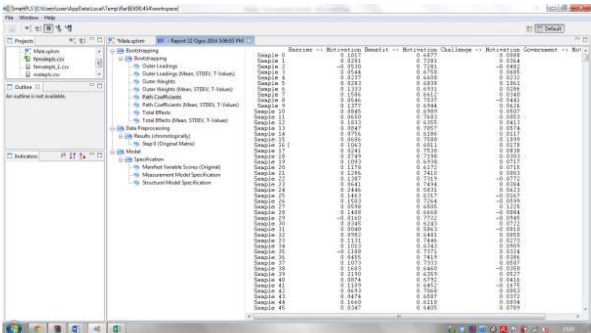
Figure 4: Female (Bootstrap)
