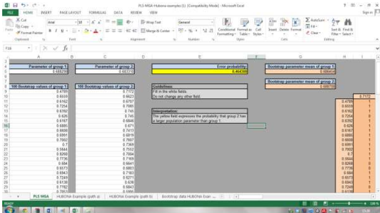
Figure 5: Non-Parametric Test
