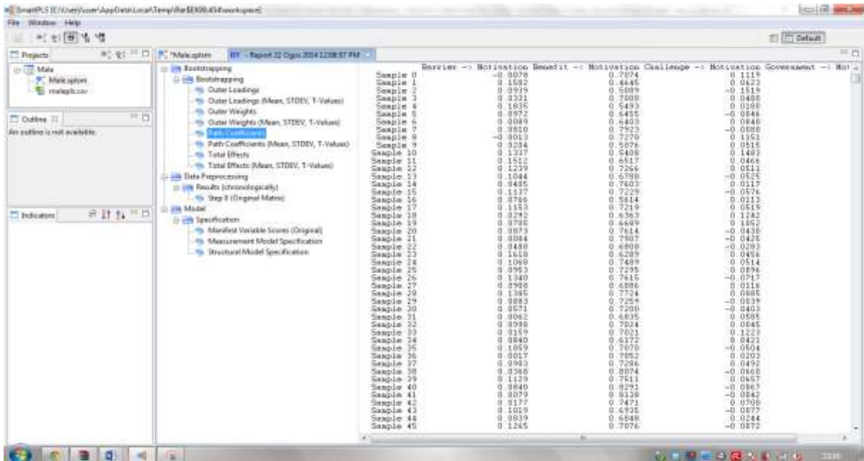
Figure 3: Male (Bootstrap)
