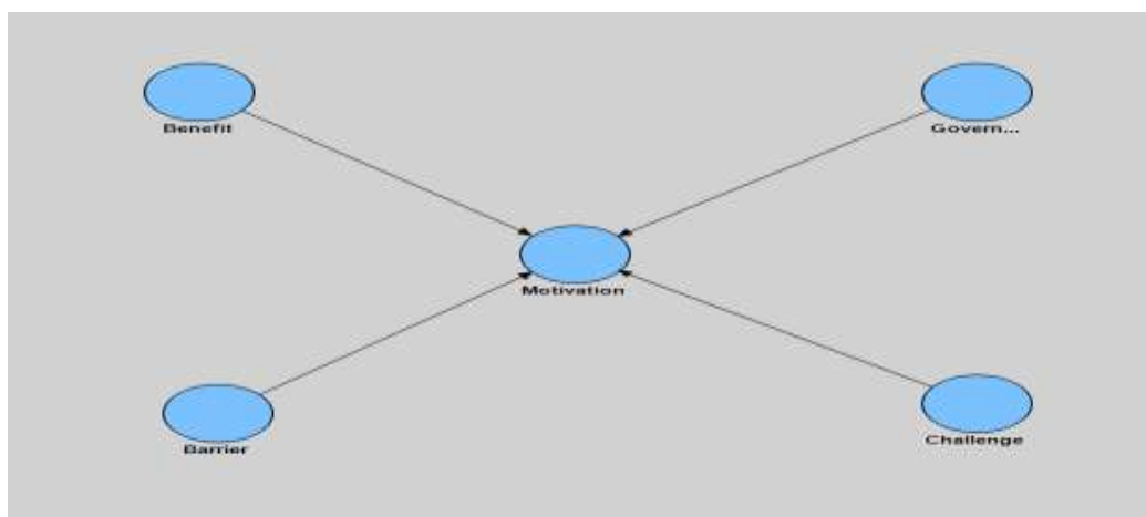
Figure 1: Theoretical Framework
