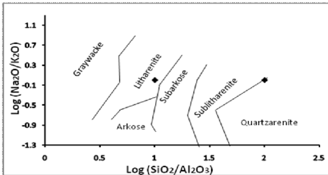
Figure 7. The plot of \log \text{Na}_2\text{O}/\text{K}_2\text{O} versus \log (\text{SiO}_2/\text{Al}_2\text{O}_3) .
