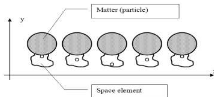
Figure 1. Time impulses given in generally as hits of space on matter. In our time: matter is always mass.
