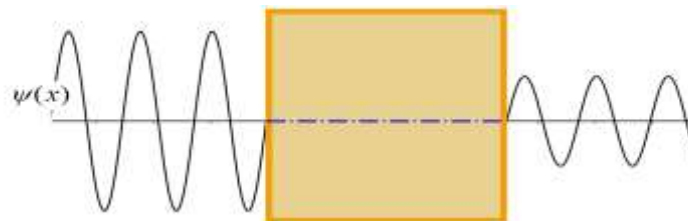
Figure 6. The wave function of tunneling particle.
