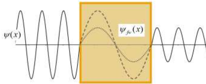
Figure 7. The function inside the barrier is a fast wave \psi_{fw}(x) . We know the frequency of the fast wave, but don't know its amplitude.
