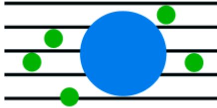
Figure 3. There are two different three-dimensional spatial dimensions depending on the actions of the objects (model, not proportional).
