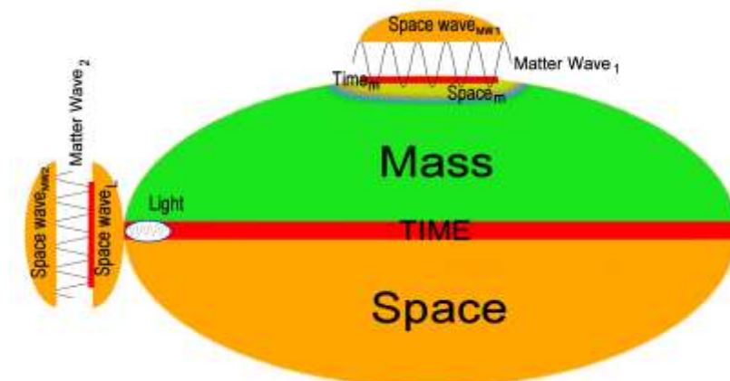
Figure 4. Space-matter model displayed as Lajtner-submarine (not proportional).
