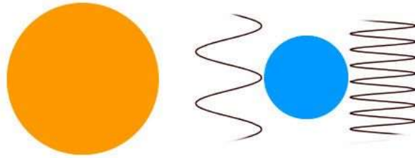
Figure 8. Space wave model of gravity (model, not proportional). Big (yellow) and small (blue) masses and space waves.
