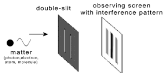
Figure 5. Double-slit experiment, model, not proportional.
