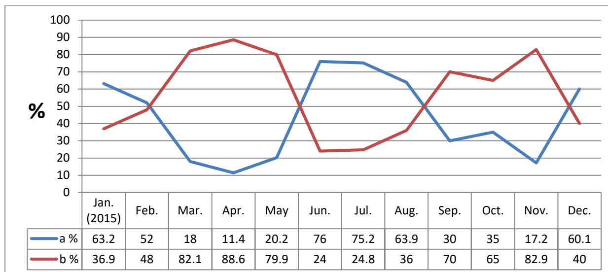
Fig. 9. Monthly variations (% by volume) in the intensity of feeding of L. sceleratus in Ain El-Ghazala Lagoon. a%: low feeding intensity, b%: high feeding intensity. The feeding intensity of Ain El-Ghazala L. sceleratus (Table 3 and Fig. 10) was high during spring (83.5%) and autumn (72.6%) and low in winter (41.6%) and summer (28.3%). Summer is the breeding season of this fish. During summer most of the abdominal cavity is occupied by gonads and so there is not enough space for the stomach when it is full with food.
