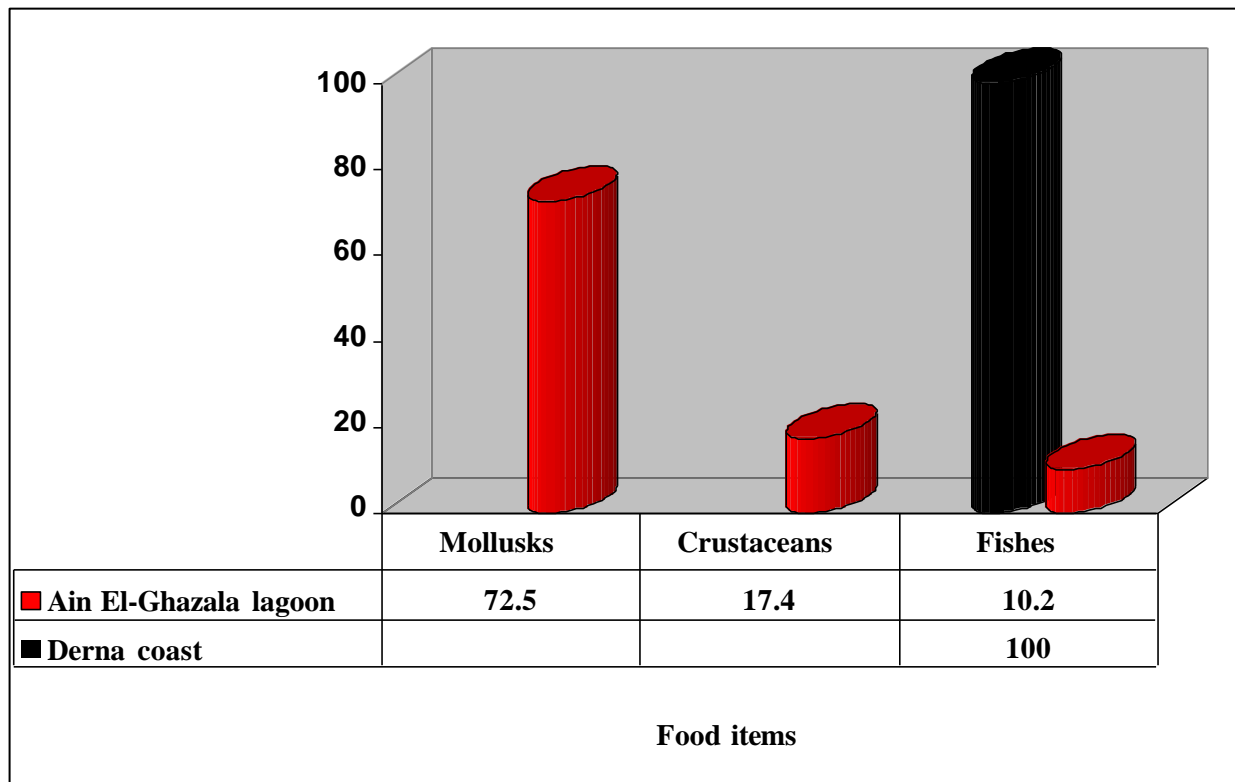
Fig. 5. Diet composition (% by volume) of L. sceleratus in Ain El- Ghazala lagoon (red bars) and in Derna coast (black bar).
