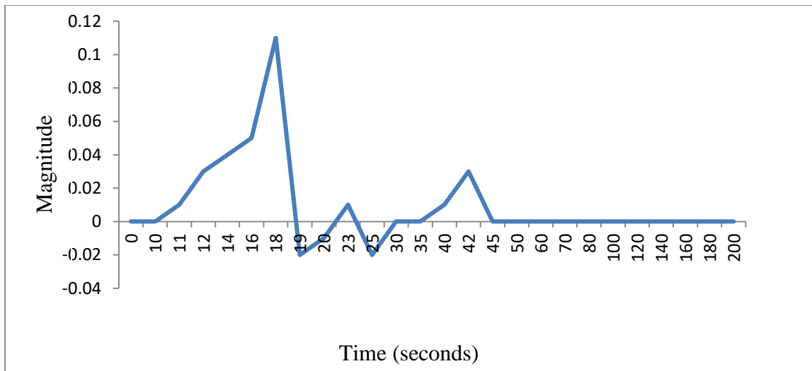
Figure 2: Impulse Response of Channel P 1
