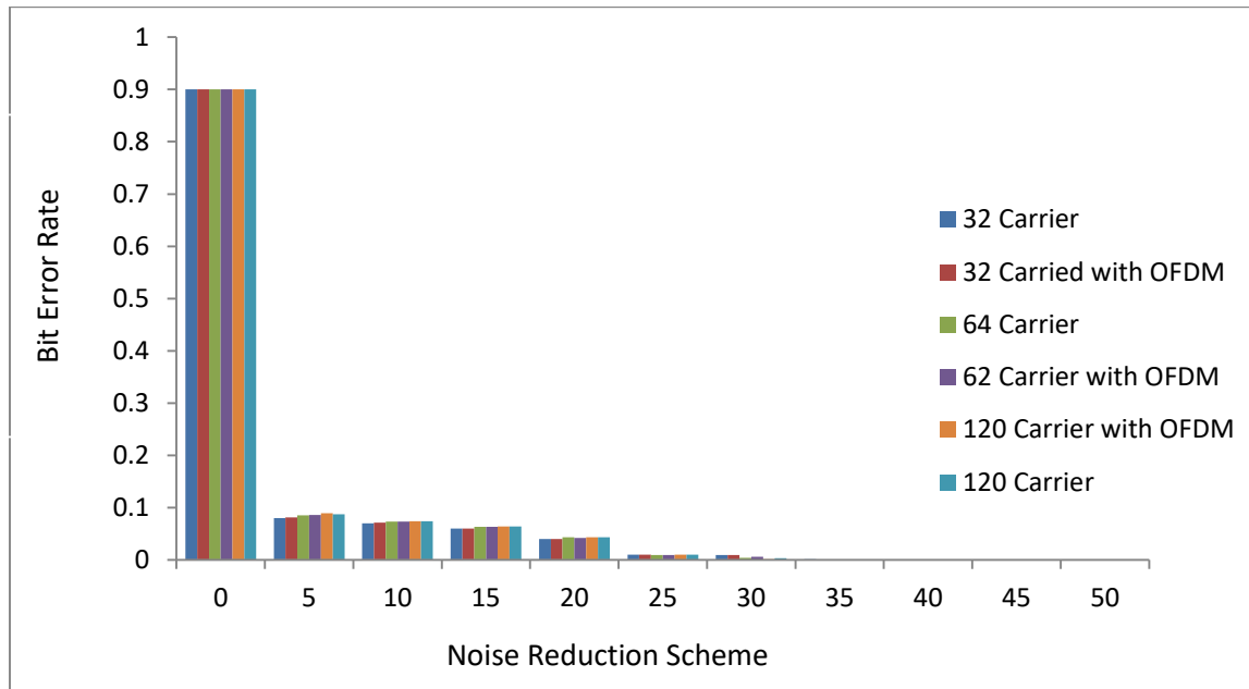
Figure 5: BER Performance of OFDM System under Multipath Effects
