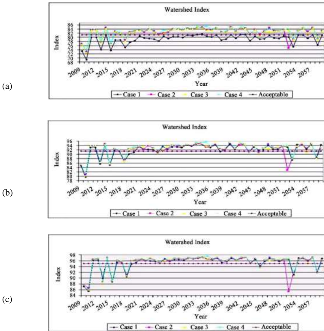
Figure 10. Watershed Index for the four land use scenarios plotted over 50 years (a) All indicators; (b) Without biodiversity indicator; (c) Without biodiversity indicator and weightage—Domestic—22, Livelihood—22, Ecological—22, Pollution—17, Energy—17.
