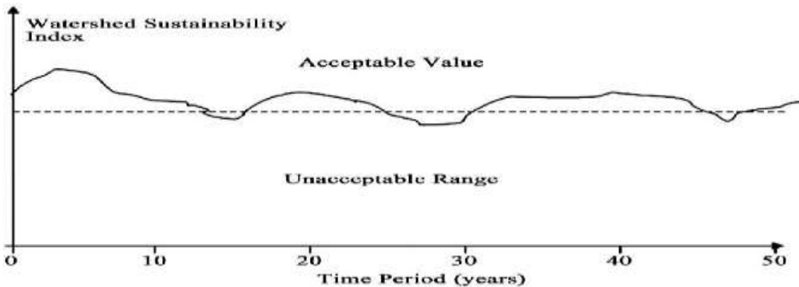
Figure 2. Watershed Sustainability Index (WSI) against time.
