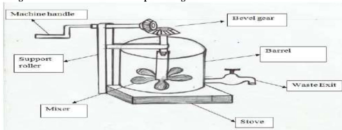
Figure 1. Manual Textile chemical mixing and processing machine (Design by Author)
