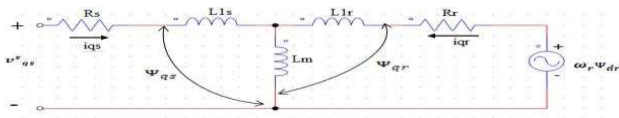
Figure 2: Equivalent circuit in quadrature axes referred to the stationary reference frame
