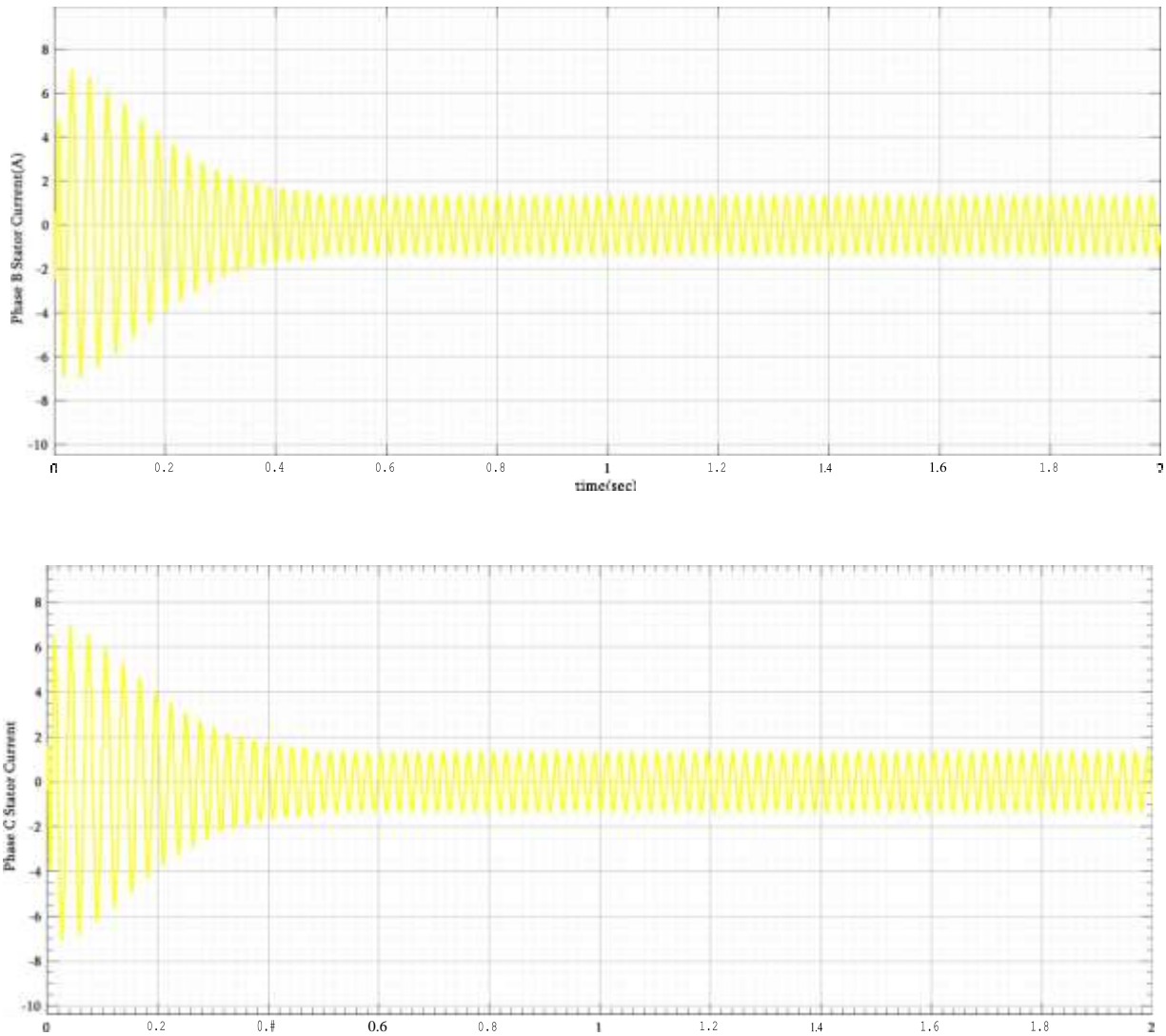
Figure 12: Stator three-phase currents MATLAB Simulink results
