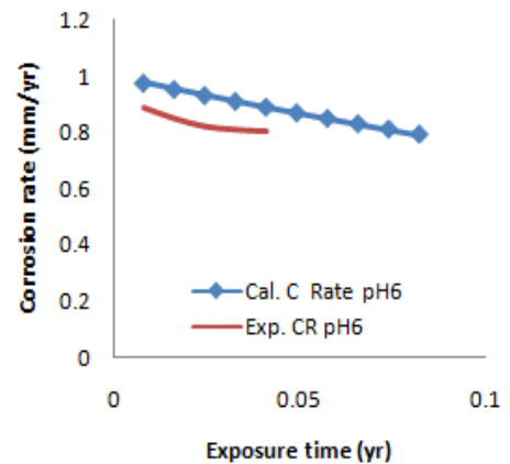
Figure 4 Variation of corrosion rate with exposure time at pH6 as Obtained from experiment compared with Model 1-predicted data
