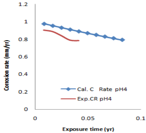
Figure 2 Variation of corrosion rate with exposure time at pH4 as obtained from experiment compared with Model -predicted data
