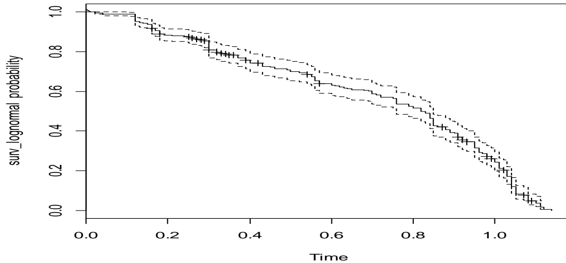
Figure 2: Survival Plot of HIV patients with opportunistic infections in Anambra State for the Lognormal Distribution
