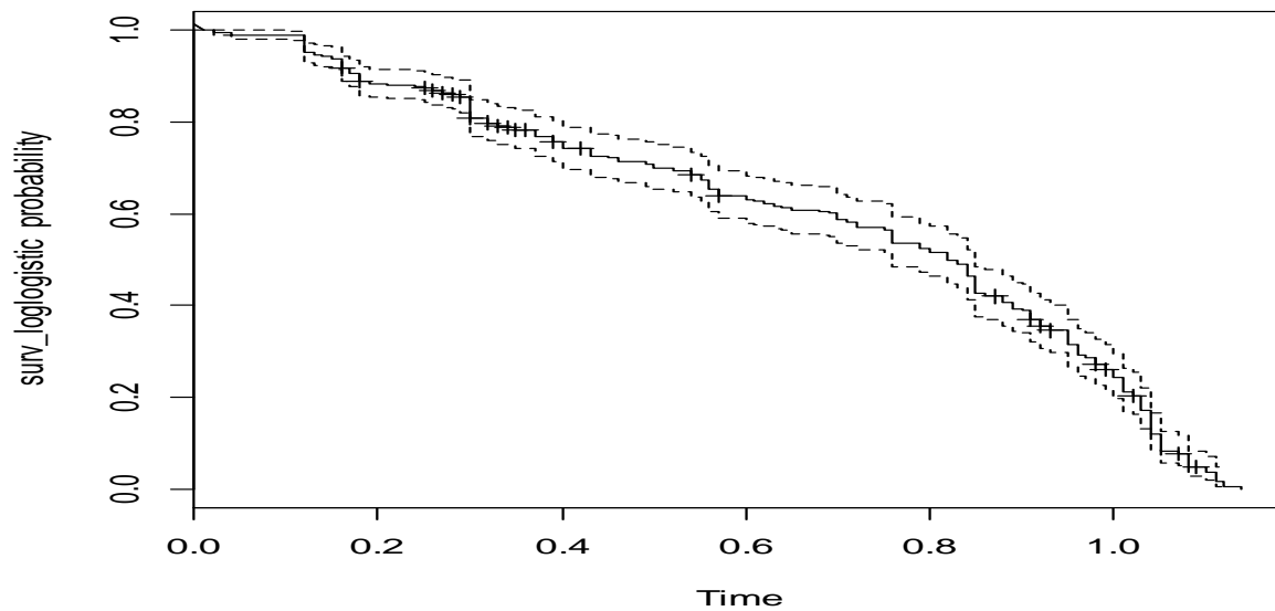
Figure 3: Survival Plot of HIV patients with opportunistic infections in Anambra State for the Loglogistic Distribution
