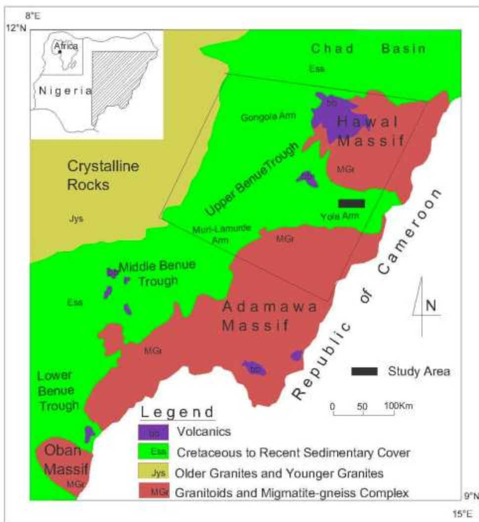
Fig. 1 Regional geologic map of Northeastern Nigeria (modified after Maluski et al. 1995).
