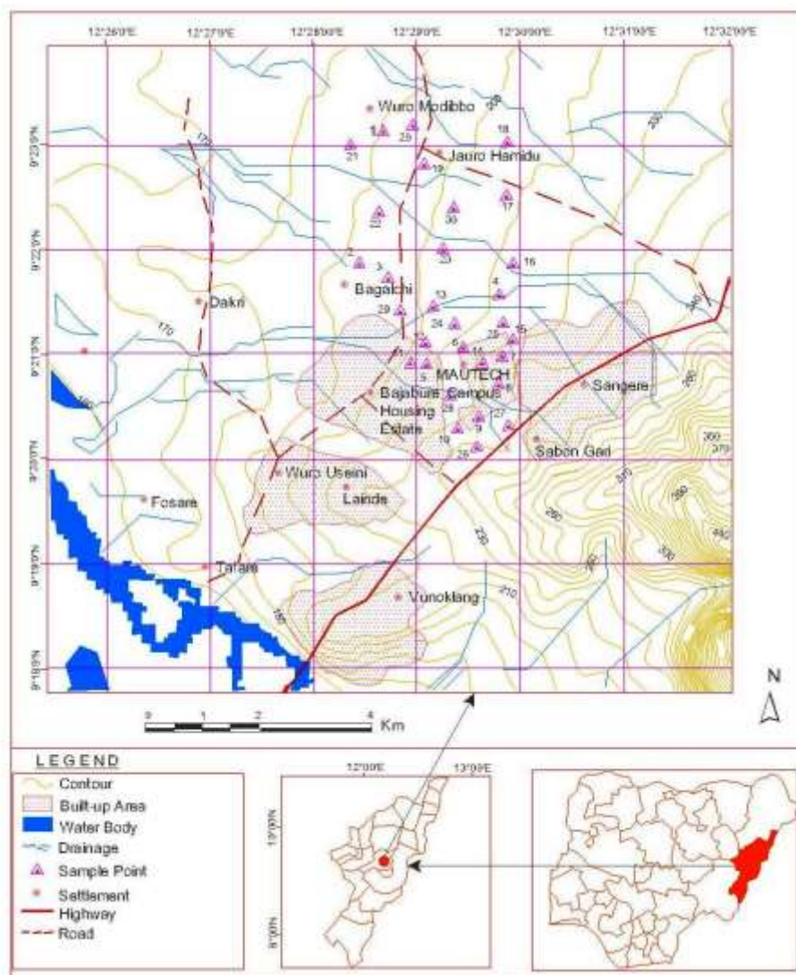
Fig. 3 Map of MAUTECH Campus and the neighbouring villages (modified from FSN, 1970).
