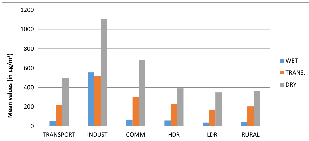
Fig. 2: Mean seasonal variations in the concentration of TSP at various landuse areas of Port Harcourt.
