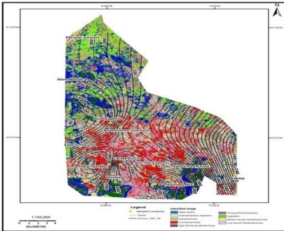
Fig. 4: TSP concentration (in \mu\text{g}/\text{m}^3 ) during transition period
