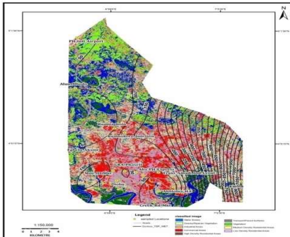
Fig. 5.: TSP concentration (in \mu\text{g}/\text{m}^3 ) during wet season (August – September, 2010).
