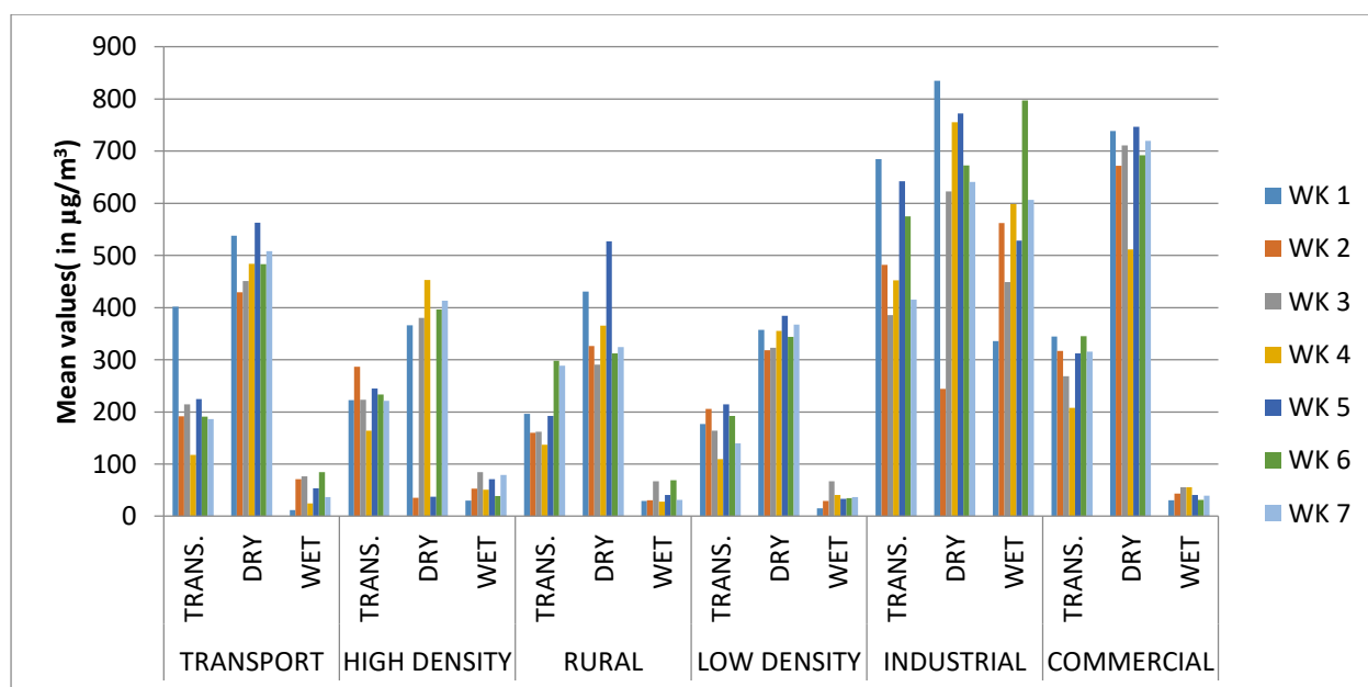
Fig 1: Mean weekly variations in the concentration of aerosol in various landuse areas of Port Harcourt
