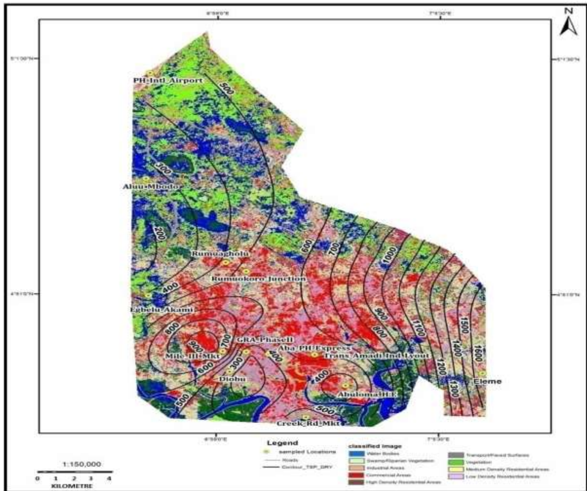
Fig.3: TSP concentration (in \mu\text{g}/\text{m}^3 ) during dry season
