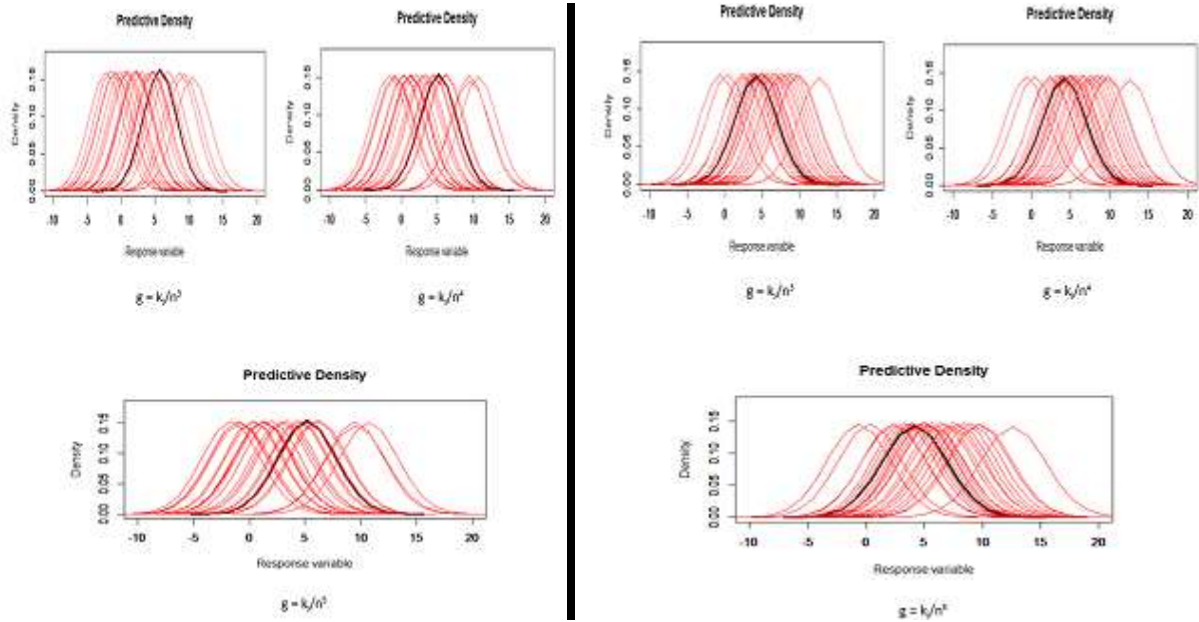
Figure 1: Point Prediction with the Modified g -priors for n=50 and n=100
