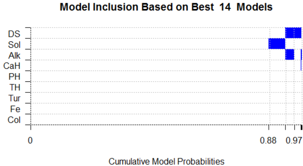
Figure 6: Cumulative Model Probabilities with the Signs of their Regressors
