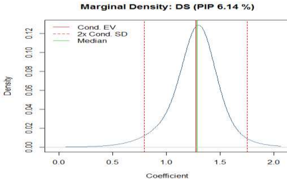
Figure 5: Marginal Density for Dissolved Solid
