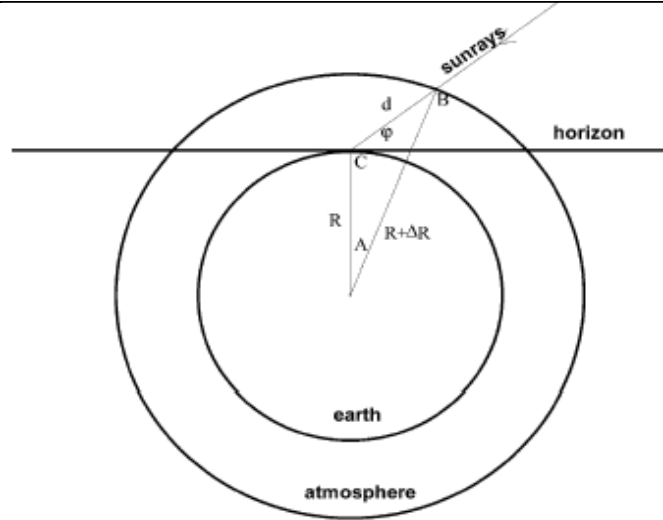
Figure 6. A schematic representations of the earth and its atmosphere with sunrays falling at an inclination \phi with respect to the horizon.
