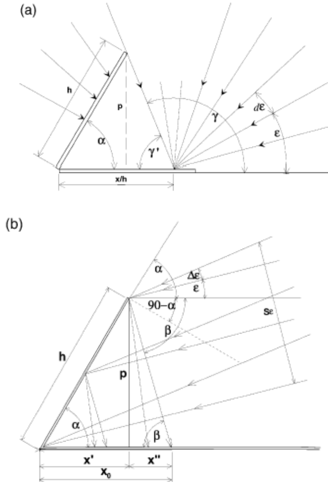
Figure 5. Schematic representations of (a) diffuse light falling onto a point at distance x/h from the reflecting wall, and of (b) diffuse light reflected by the wall.
