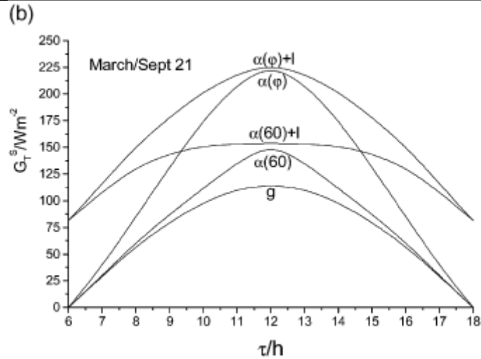
Figure 9. Calculated dependence of ground irradiance on time for the shortest day of the year and for equinox in a greenhouse with a reflecting wall inclined at an angle of 60^\circ , ( \alpha(60) ) with a reflecting wall with variable inclination ( \alpha(\varphi) ), without louvers and ( \alpha(60) + 1 ), ( \alpha(\varphi) + 1 ) the same but with louvers.
