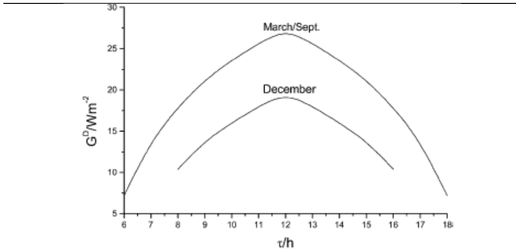
Figure 12 Ground irradiance from diffuse (sky) radiation from a clear sky at the shortest winter day and at equinox.
