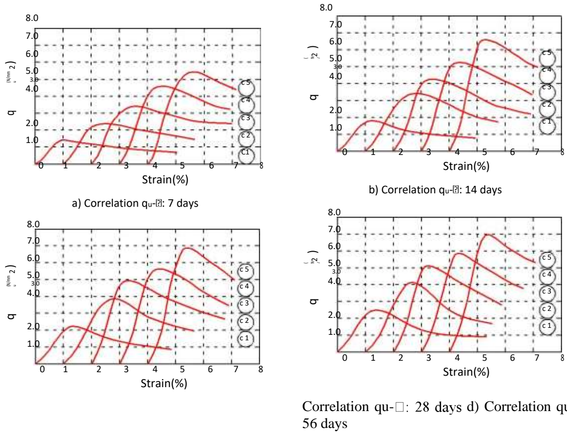
Figure 3. Unconfined compressive strength - strain of laboratory stabilized soil
