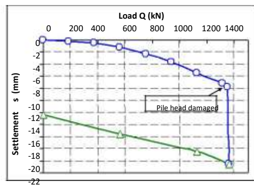
Figure 13. Result of load- Settlement for TP02
