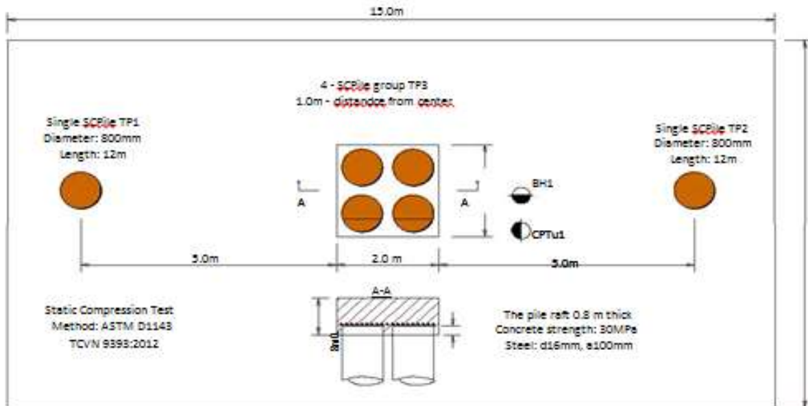
Figure 10. Schematic presentation of the test geometry
