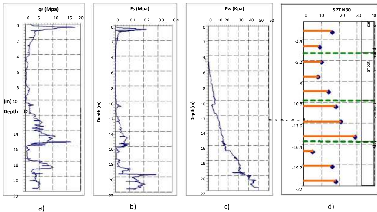
Figure 2. Measured data from CPTu test and SPT test
