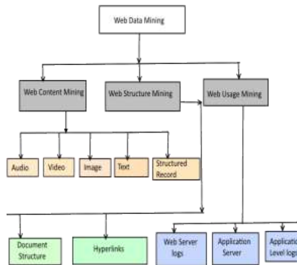
Fig. 1. Web data mining system structure.
