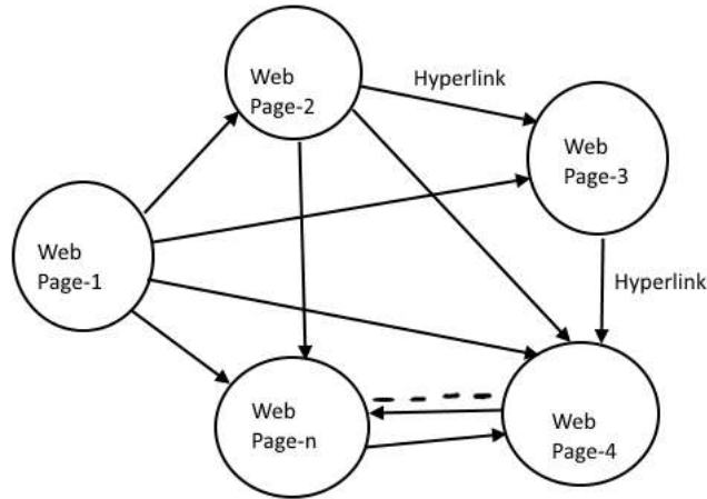
Fig. 2: Web structure mining as a graph.
