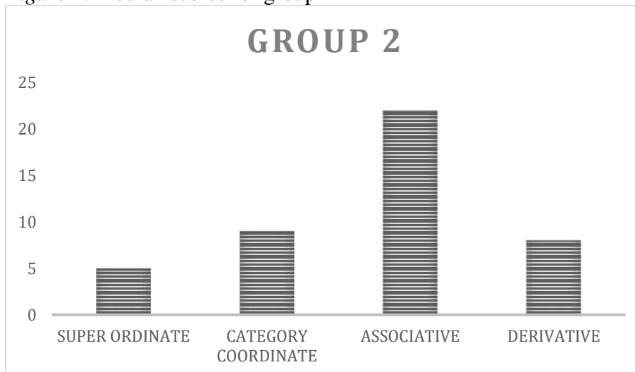
Figure 2. Median scores for group 2
