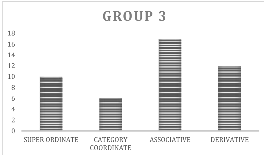
Figure 3. Median scores for group 3.
