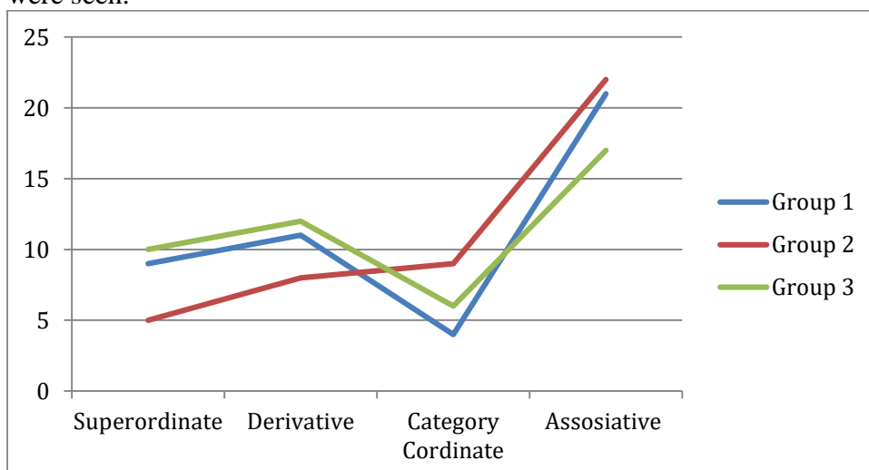
Figure 4. Pattern of the four semantic ordinates for the three groups.
