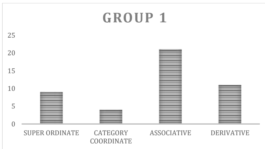
Figure 1. Median scores for group 1
