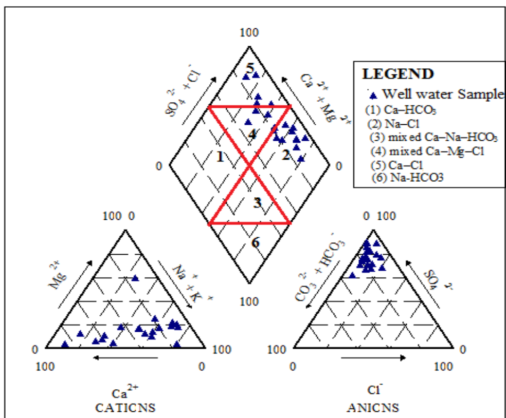
Fig. 2. Piper Diagram of Well Water Samples from the Study Area
