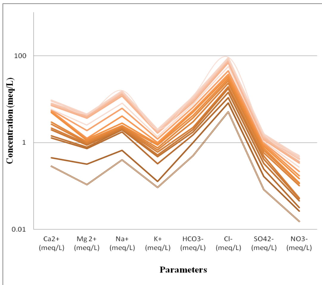
Fig. 3. Schoeller Diagram of Well water from the Study Area
