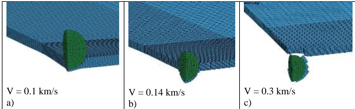
Figure 3: Impact simulation on an Al plate of 0.08128 cm thickness: a) non-penetration; b) penetration occur/penetration limit; c) full penetration.
