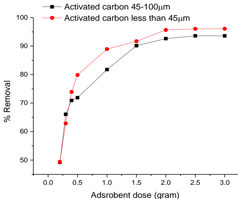
Figure3. Effect weight of adsorbent active carbon (100-45um) and (less than 45µm) on adsorption capacity, 20.08ppm dye concentration, connect time 120 min and at 25°C.
