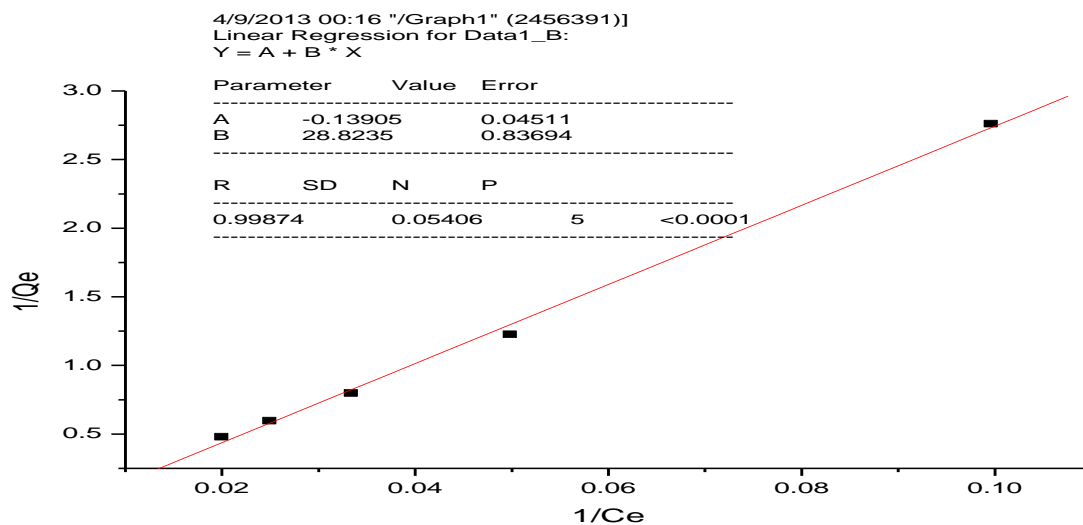
Figure 8. Freundlich isotherm for acid red 186 adsorption onto 1g active carbon (100-45um) at 25°C.
