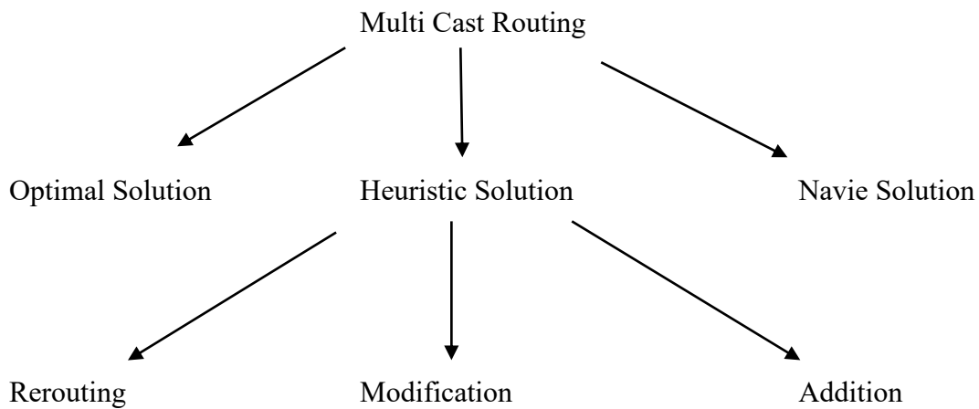
Fig 3: Multicast Routing
