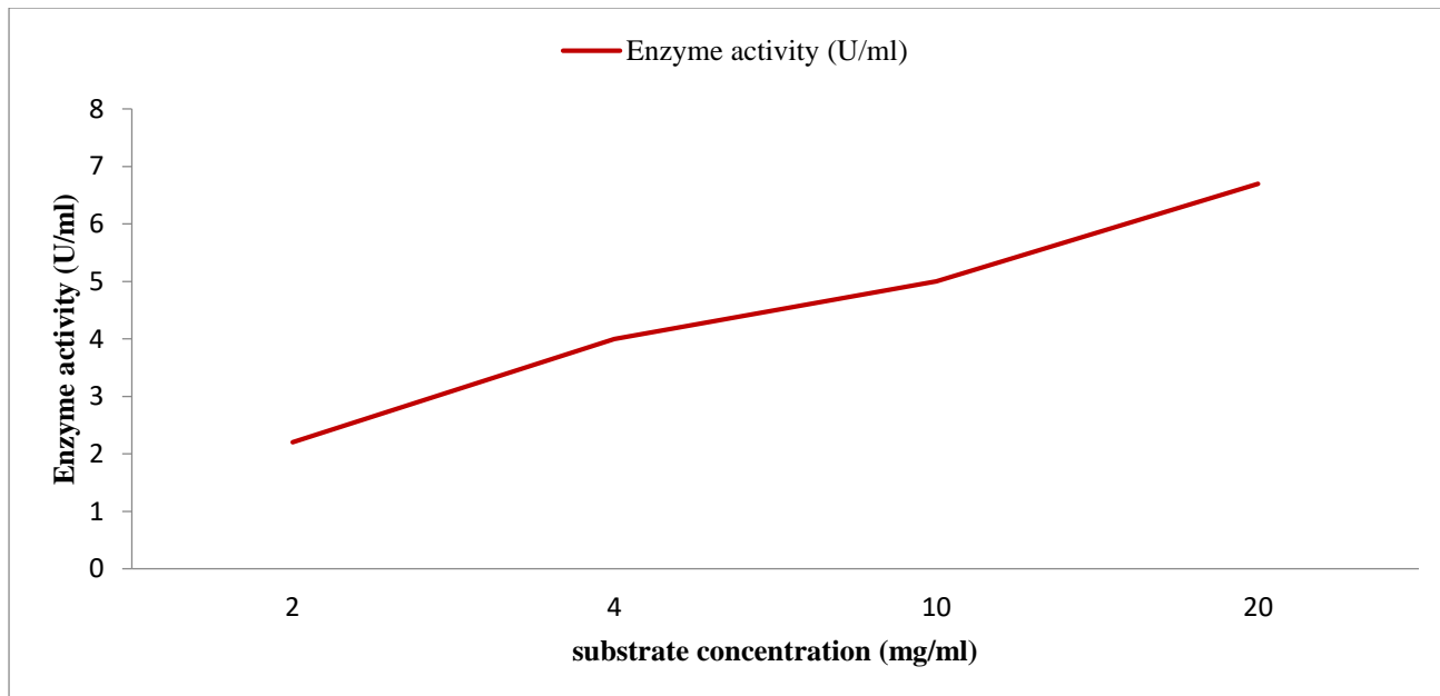
Figure 5: The effect of substrate concentration on Pseudomonas aeruginosa IZ cellulase activity
