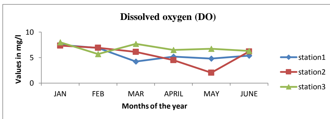
Fig-7: Monthly variation in Dissolved Oxygen of Okhuo River, Edo State.
