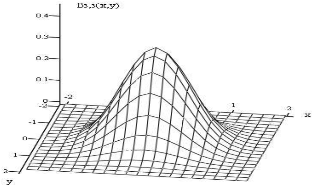
Figure 2. Two-dimensional spline basis of the third degree.
