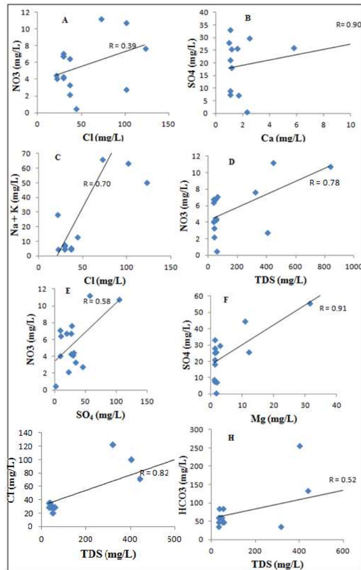
Figure 4. Variation diagrams of some ions in water samples of the Study Area
