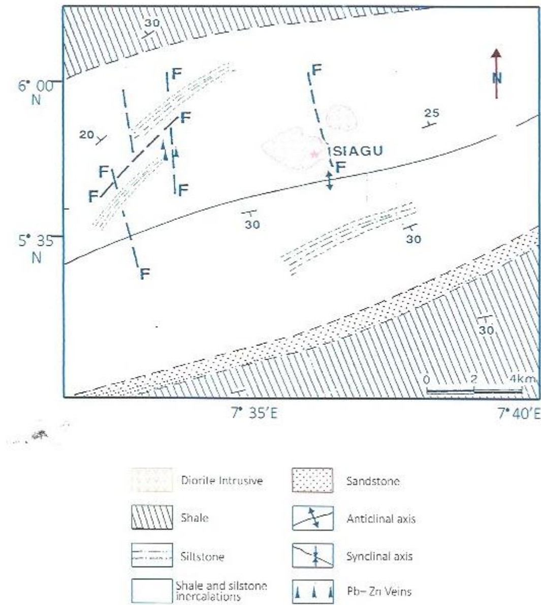
Fig. 4: Geology and lead-zinc veins at Isiagu (Modified after Olade 1976)
