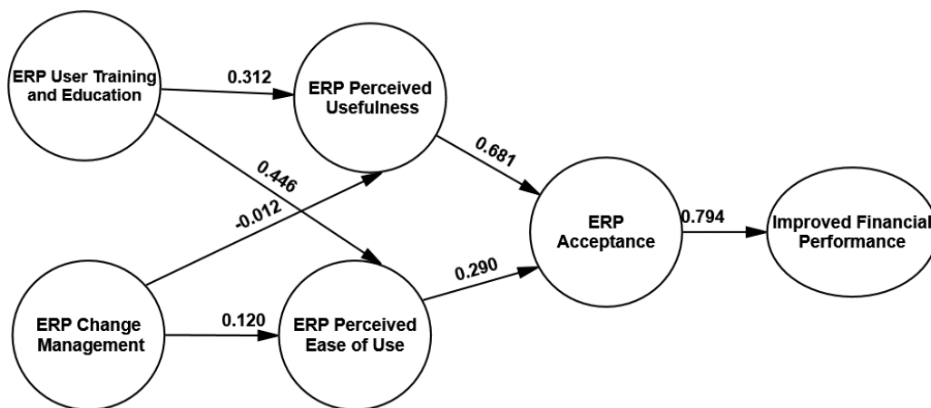
Figure 2: path testing
