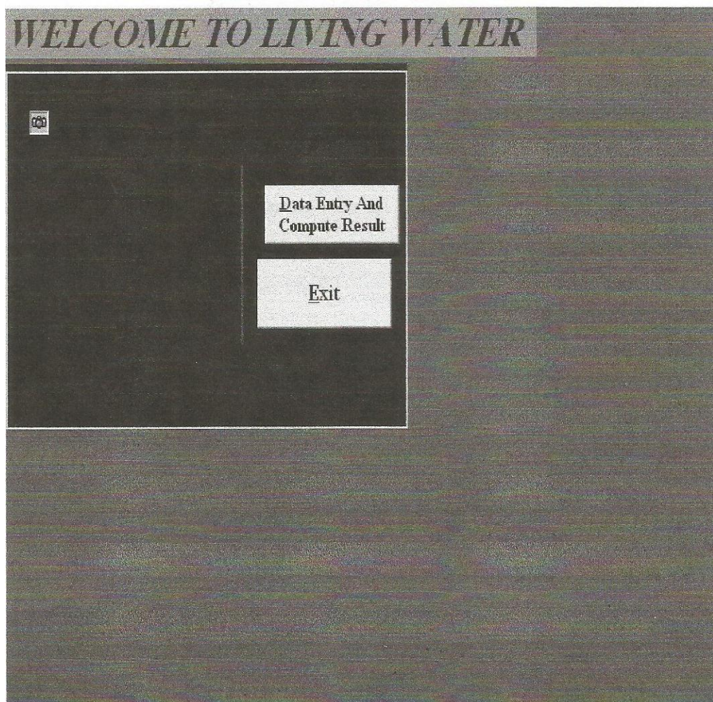
Figure 1.1: FrmMain
