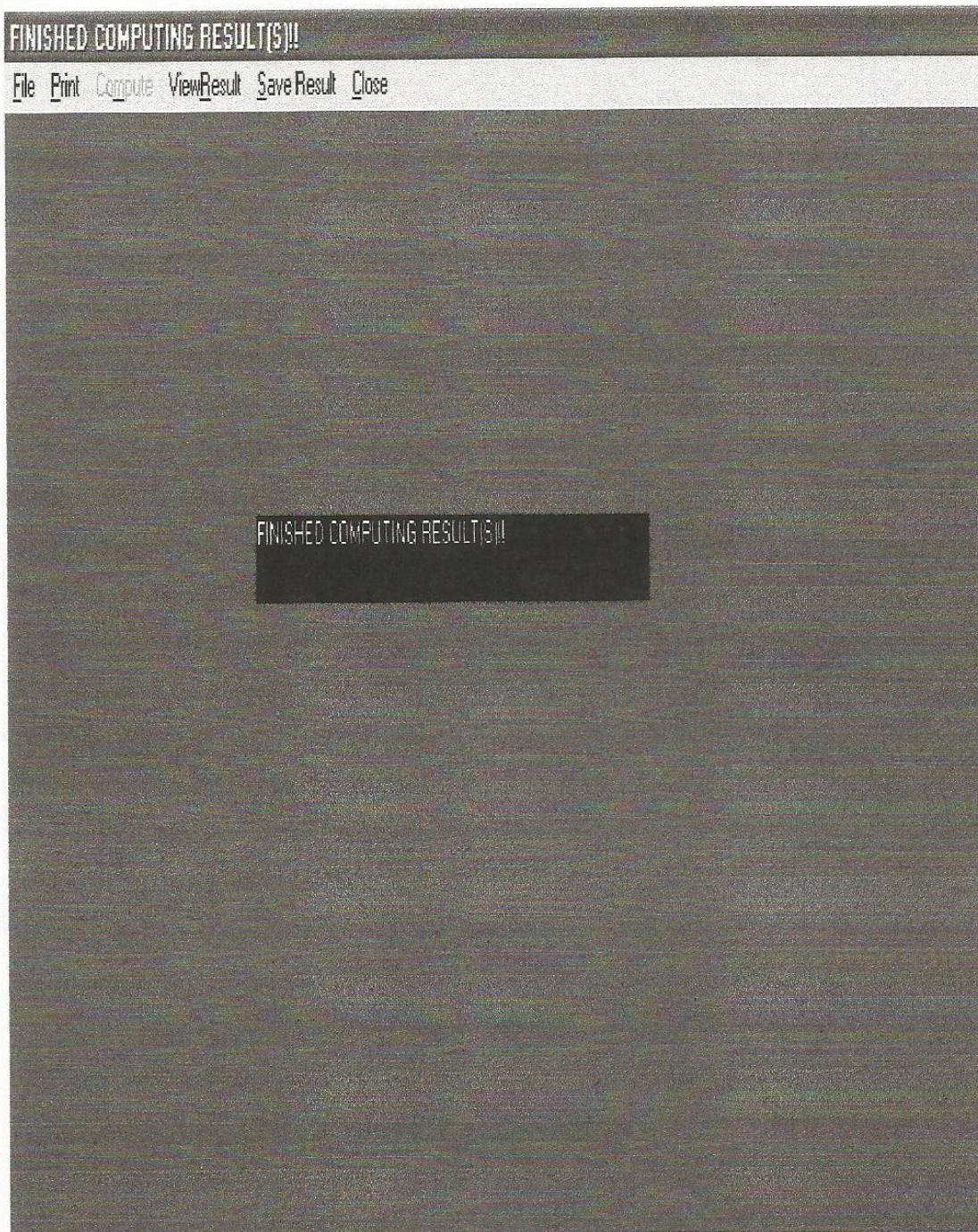
Figure 1.3:FrmView
