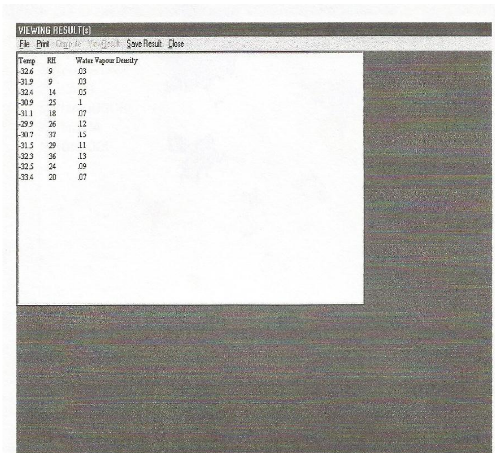
Figure 1.4 Calculated result
