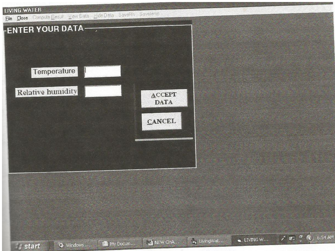
Figure 1.2:FrmtempRh
