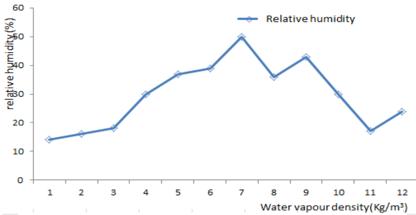
Figure 1.1 b Variation of relative humidity against water vapour density
