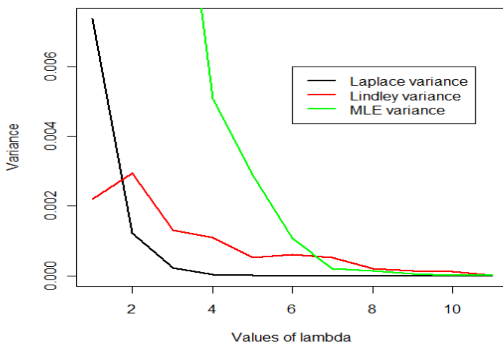
Figure 4: Graph of variance for sample size 100 against values of Lambda ( \lambda ).
