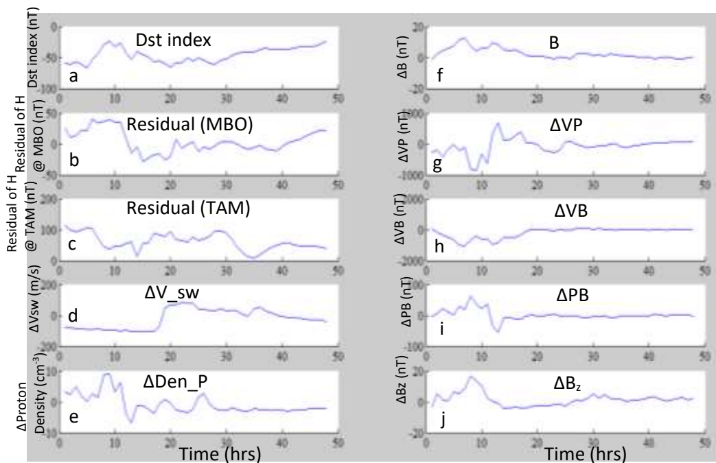
Fig. 2: Time series of hourly (a) Dst index and the hourly mean of (b) residual H – component in MBO, (c) residual field at TAM, (d) V_{sw} , (e) \text{Den}_P , (f) B, (g) VP, (h) VB, (i) PB, and (j) B_z of IMF for the storm days of 4 th – 5 th of August, 2004.
