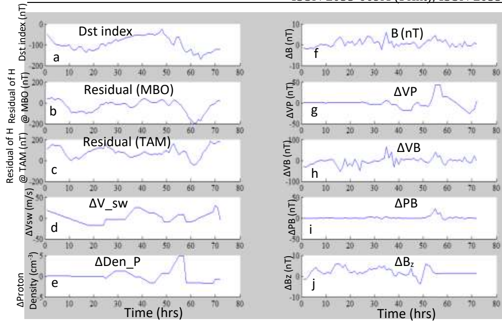
Fig. 1: Variation of (a) Dst index and the hourly mean of (b) residual H – component in MBO, (c) residual field at TAM, (d) V_{sw} , (e) \text{Den}_P , (f) B, (g) VP, (h) VB, (i) PB, and (j) B_z of IMF for the storm days of 25 th – 27 th July, 2004.
