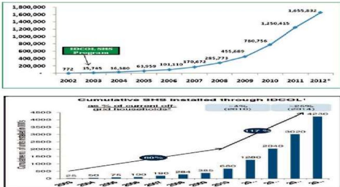
Fig 4: (Top) SHS installations from 2003 to 2012, IDCOL; (Bottom) Cumulative number of targeted SHS installations till 2014 [4].
