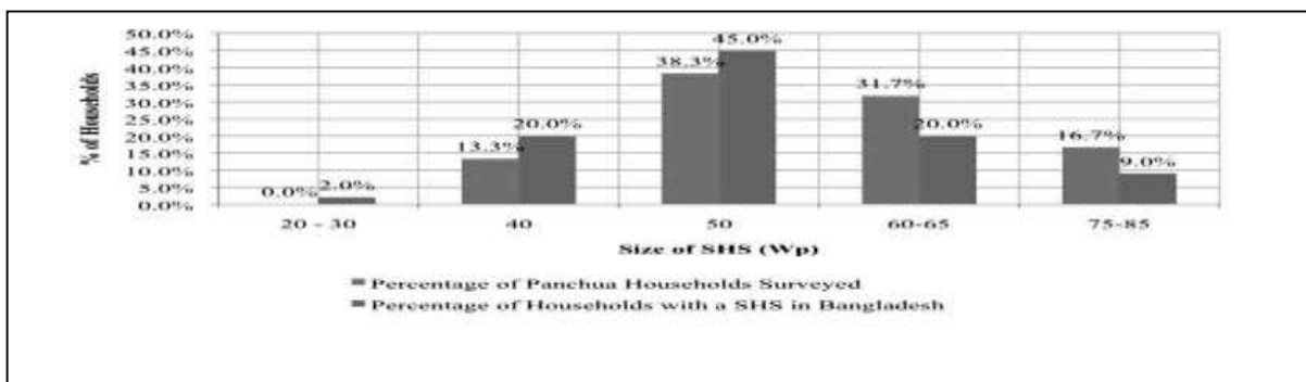
Fig.7. Comparative breakdown of SHS size in Panchua Village and across Bangladesh.
