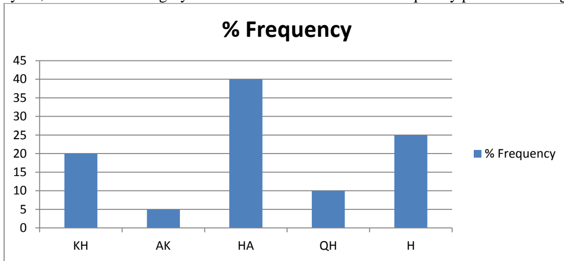
Figure 2. Bar Chart of the VES Curve types of the study area.
