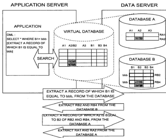
Figure: Extracting data using VDB
