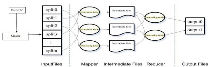
Figure: MapReduce execution flow with VDB
