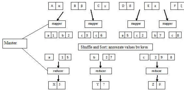
Figure: Simplified view of MapReduce
