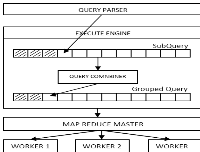
Figure: Query Optimization
