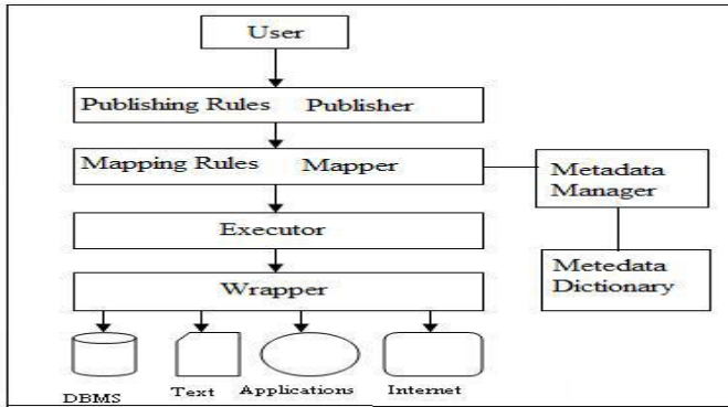
Figure: Virtual Database System-General structure
