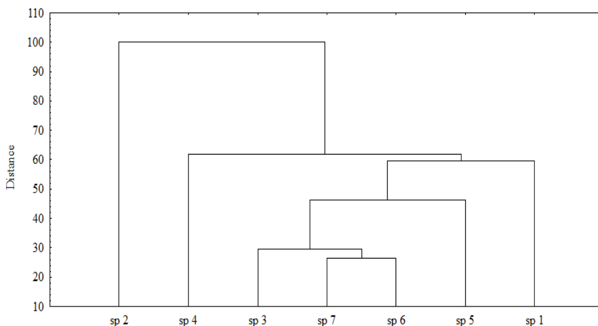
Fig 5. UPGMA- phenogram based on 34 taxonomic characters obtained from different studies for different taxa.
